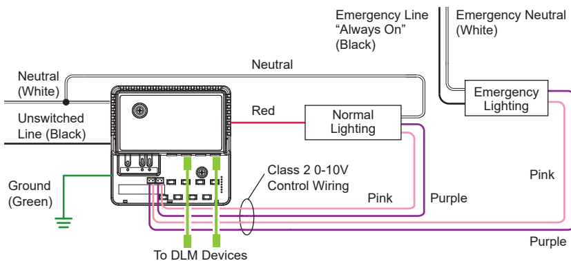
Load A ON/OFF/Dim
