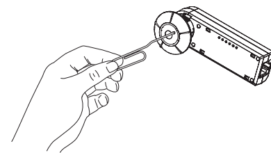
Fig. 9: CONFIG Button
