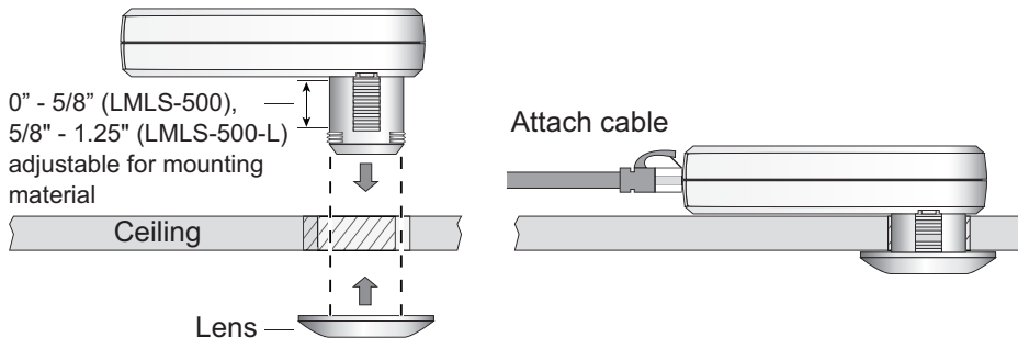
Fig 3: Mount Sensor to Ceiling
