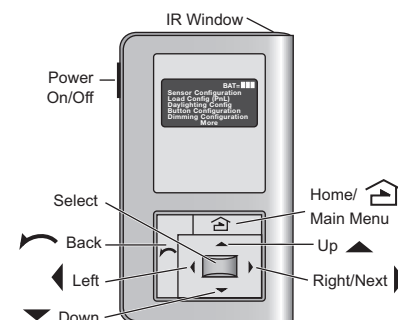
Fig. 12: LMCT-100 Controls
