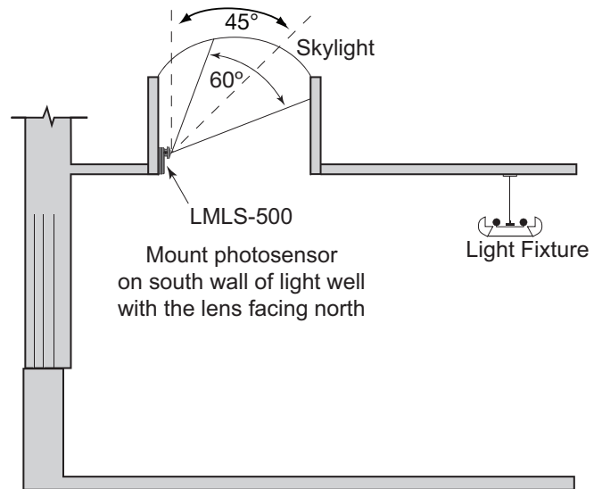
Fig. 1b: Skylight Location
