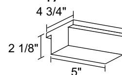
Canopy Transformer
