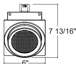
Louvered Version
