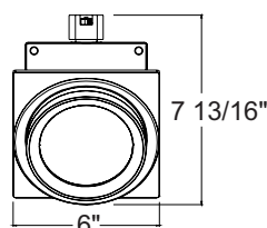
Non-Louvered Version
