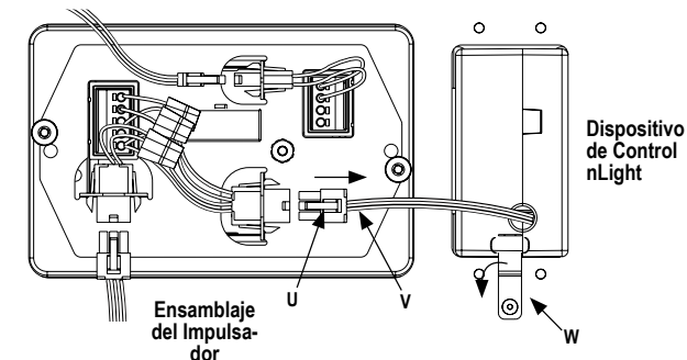
Fig. 13b: Carcasas AX3(SQ) LPA/LPD
