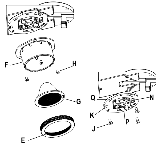
Fig. 11b: Dedicated Wall Wash Housing
