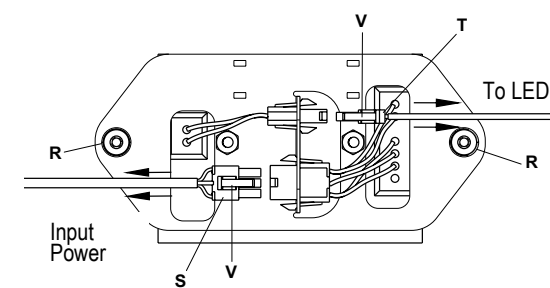
Fig. 12b: AX3(SQ) LPA/LPD Housings
