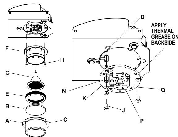
Fig. 11a: AX3(SQ) Housings
