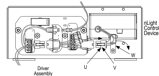
Fig. 13b: AX3(SQ) LPA/LPD Housings
