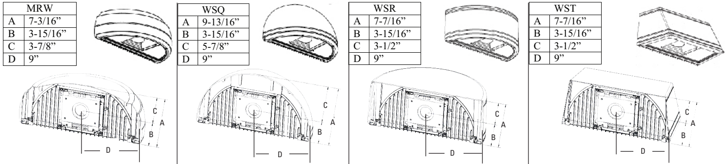
Wall mounting plate
