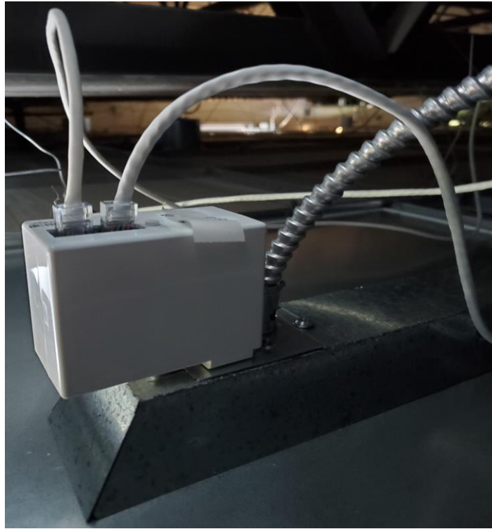
Figure 6: NPP16D Install
