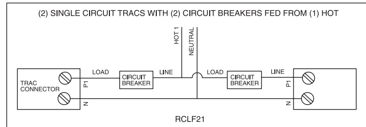
Diagram 4 (In-Line Feed)
