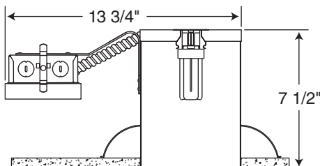
6 3/4" Ceiling Cutout
