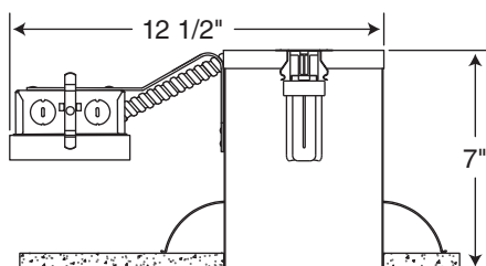
6 3/4" Ceiling Cutout
