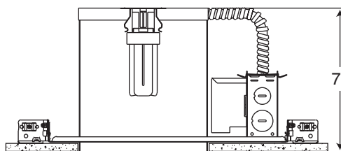
6 7/8" Ceiling Cutout
