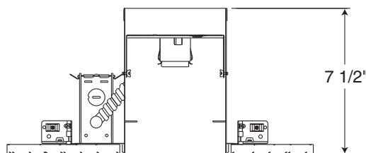
5 5/8" Ceiling Cutout
