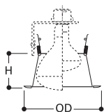
H930 R/PAR lamp aiming accessory for 310 and 426 trims. Allows 30° tilt and 358° rotation. 50W PAR30, 65W BR30, 75W PAR30, 100W R30.
