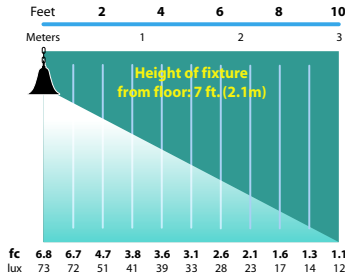
SL-05 Half Spread Photometrics 20 ft. (6.0m) diameter
