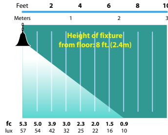
SL-05 Half Spread Photometrics 14 ft. (4.3m) diameter
