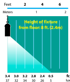
SL-14 Half Spread Photometrics 12 ft. (3.7m) diameter
