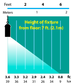
SL-14, SL-15 Half Spread Photometrics 12 ft. (3.7m) diameter
