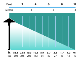
AL-16 Half Spread Photometrics 20 ft. (6.1m) diameter
