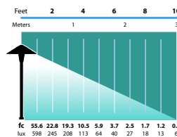
AL-15 Half Spread Photometrics 20 ft. (6.1m) diameter
