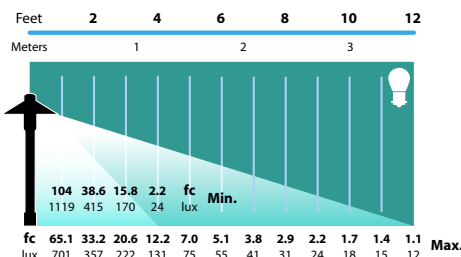
AL-13, AL-13-DM Half Spread Photometrics 8 ft. (2.4m) to 24 ft. (7.3m) diameter
