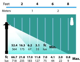
AL-13-SM Half Spread Photometrics 7 ft. (2.1m) to 16 ft. (4.9m) diameter
