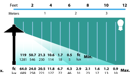
AL-13-LG Half Spread Photometrics 12 ft. (3.7m) to 22 ft. (6.7m) diameter
