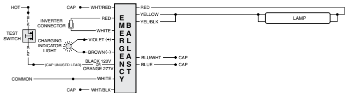
FIG I ONE (1) 32-215 W LAMP WITHOUT AC BALLAST
