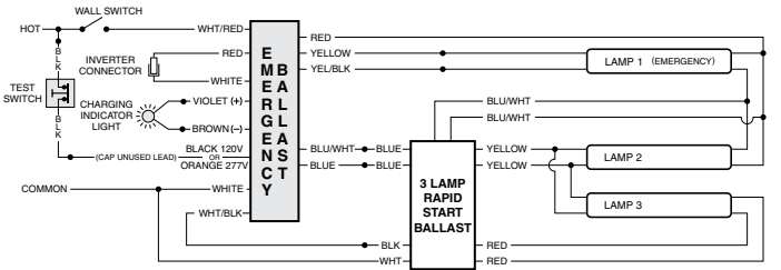
FIG F THREE (3) LAMP RAPID START BALLAST
