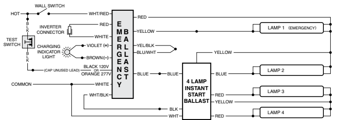
FIG G FOUR (4) LAMP INSTANT START BALLAST
