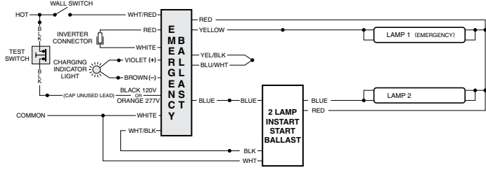
FIG C TWO (2) LAMP INSTANT START BALLAST
