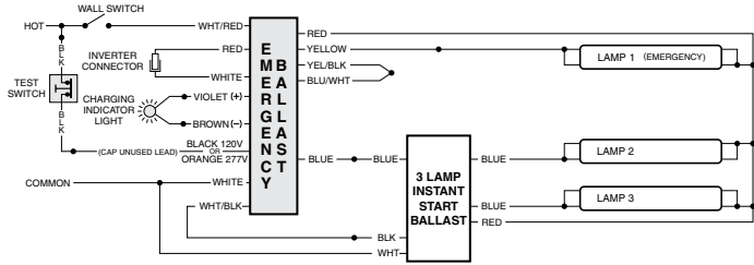
FIG E THREE (3) LAMP INSTANT START BALLAST
