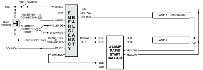
FIG D TWO (2) LAMP RAPID START BALLAST
