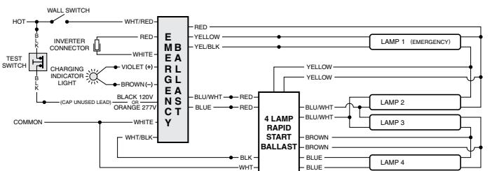
FIG H FOUR (4) LAMP RAPID START BALLAST
