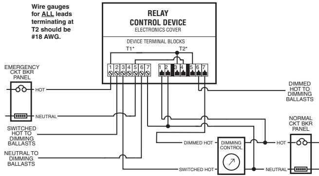
Device as an Inverter or Generator Transfer Device with a 3-wire Dimming System
