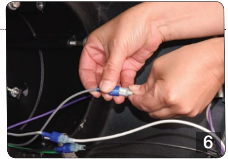
Disconnect all wires coming from arm as shown. Remove and discard existing driver assembly.
