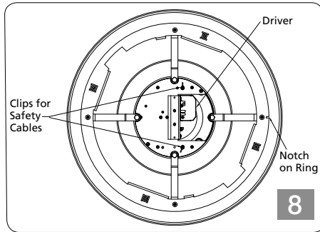
Rotate driver assembly to make sure it lines up as shown in the diagram.
