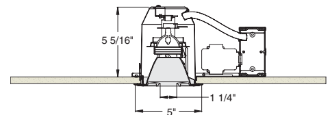
4 7/16" CEILING CUTOUT
