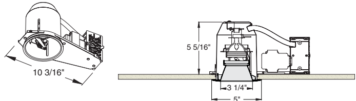
4 7/16" CEILING CUTOUT
