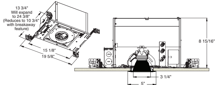
4 1/4" CEILING CUTOUT
