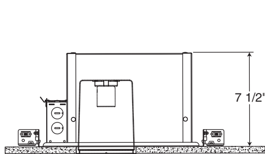
4 1/2" Ceiling Cutout
