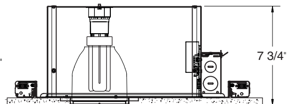
4 1/2" Ceiling Cutout
