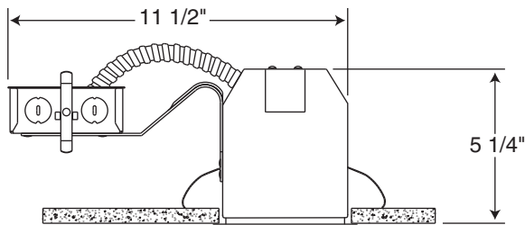
4 3/8" Ceiling Cutout
